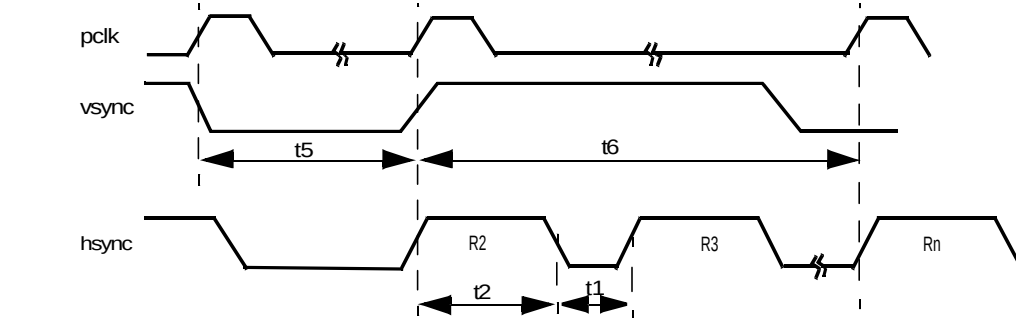
Figure 50. Frame Timing
