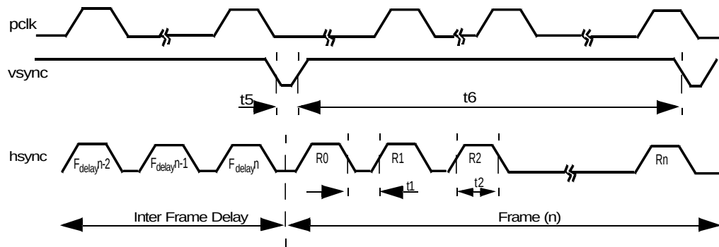
Figure 51. Frame Delay Timing (With Inter Frame Delay).
