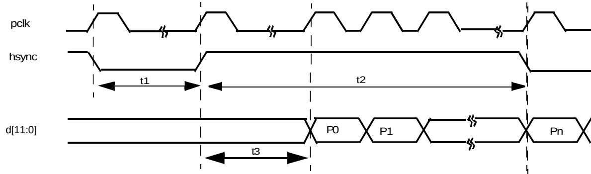
Figure 49. Row Timing Diagram
