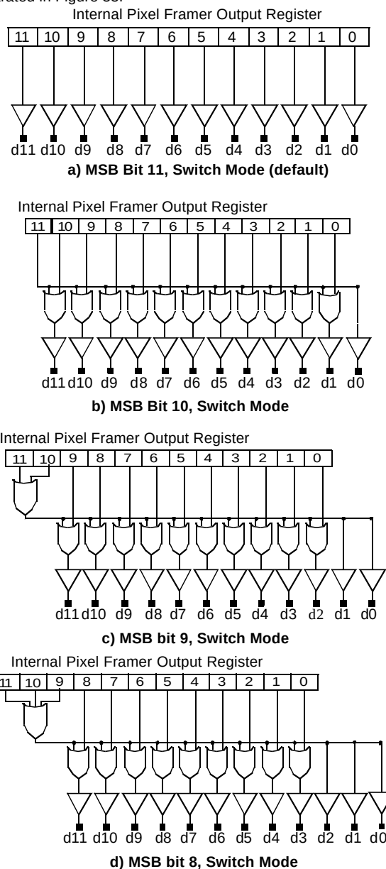
Figure 33. Digital Video Bus Switching Modes
