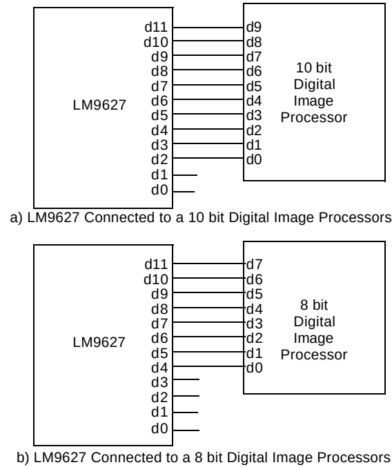
Figure 34. Example of connection to 10/8 bit systems
